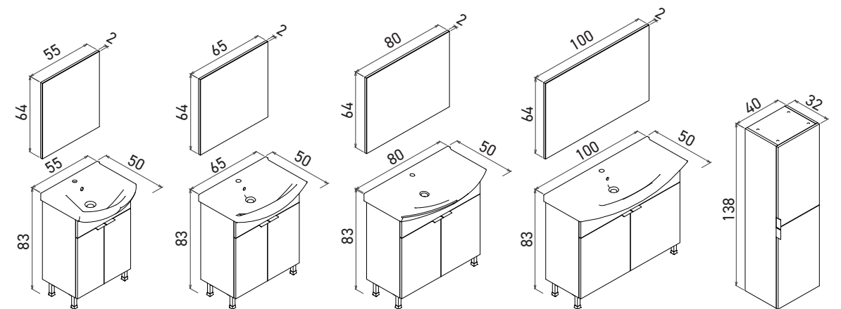
TEKNİK ÇİZİM / TECHNICAL DRAWING
