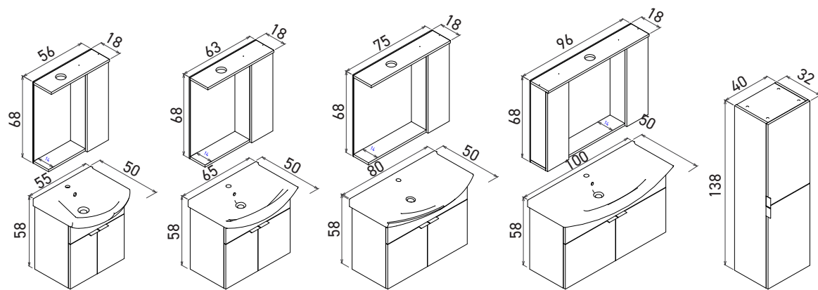
TEKNİK ÇİZİM / TECHNICAL DRAWING
